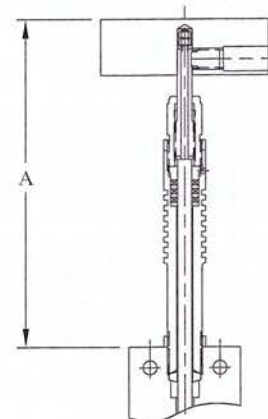
Finned Bonnet
